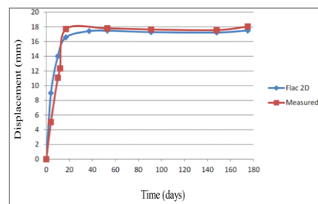
Fig. 1. Agreement between the monitored convergence data and the FLAC2D simulation results
