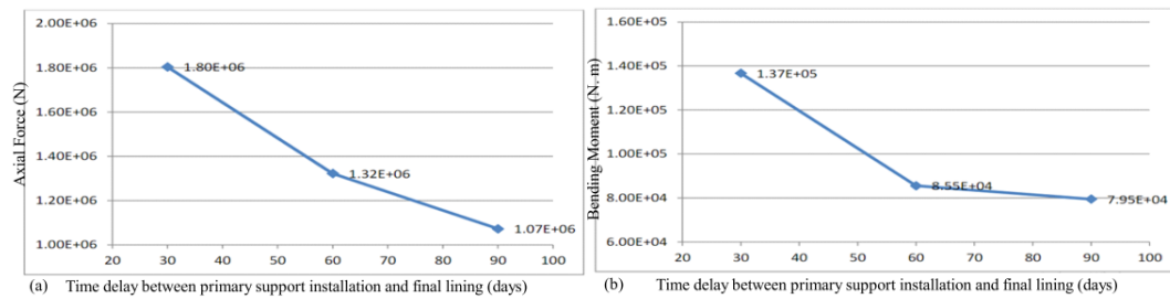
Fig. 2. Variations in (a) axial force and (b) bending moment with increasing time interval between temporary support installation and final lining placement
